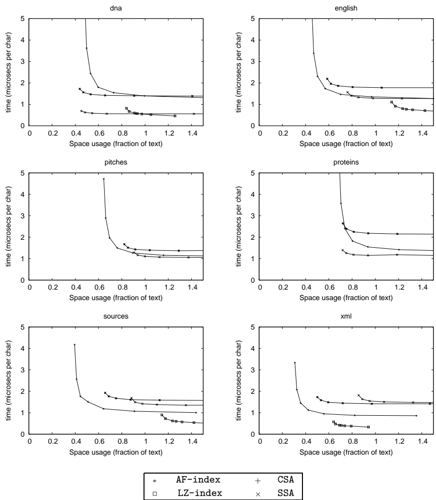
Fig. 5. Space-time tradeoffs for extracting text symbols.
